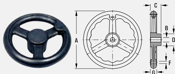
Handwheel Without Handle
