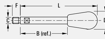
With Oval Ball Knob
