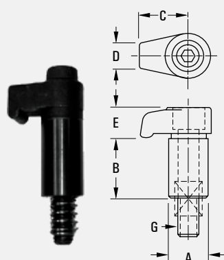
Socket Head Cap Screw Style
